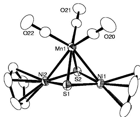
Figure 1. An ORTEP diagram of the molecular structure of \text{Cp}_2\text{Ni}_2(\mu_3\text{-S})_2\text{Mn}(\text{CO})_3 , 1 , showing 40% thermal ellipsoid probability.
